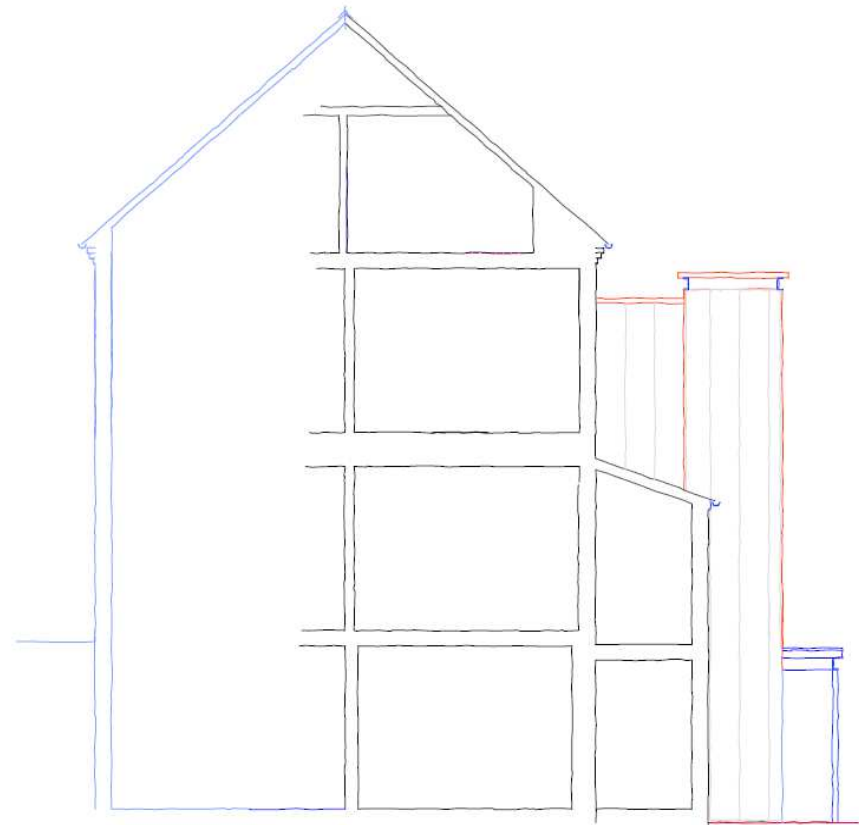
NORTH-WEST ELEVATION
